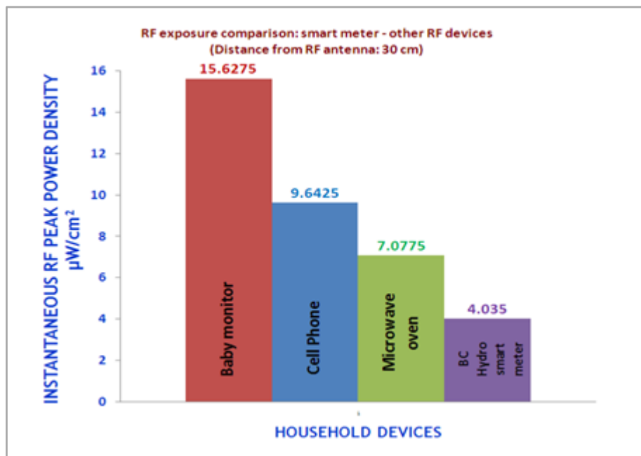
Figure 2: Measured Comparative RF Exposure at 30 cm (1 foot)
