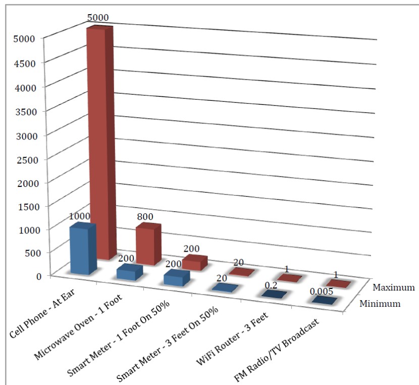
Figure 1: Comparison of Radio-Frequency Levels from Various Sources (in \mu\text{W}/\text{cm}^2 )
